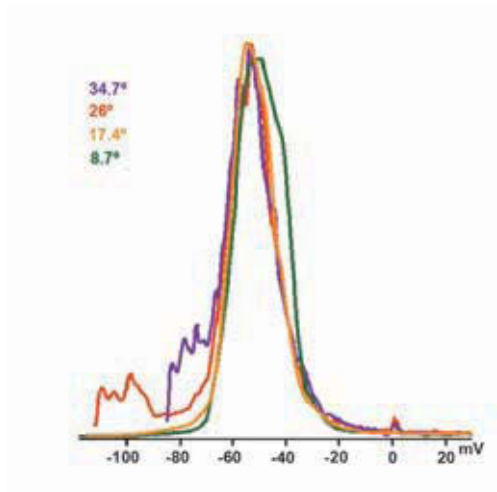
Fig. 10 – Distribution of the zeta potential for the different angles of incidence of the laser
