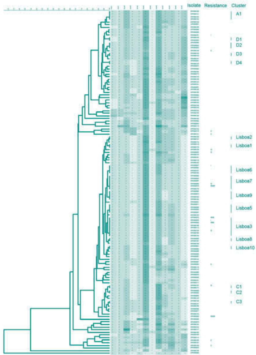
Fig. 2 – MIRU-VNTR dendrogram of the 132 M. tuberculosis clinical isolates analyzed. Resistance pattern
