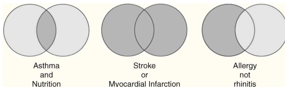
Figure 1 Boolean Operators
